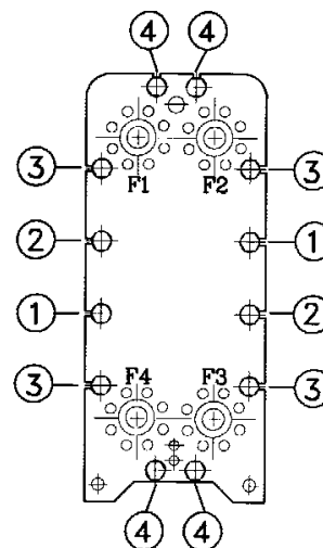
FIG. 7 : TIGHTENING SEQUENCE
